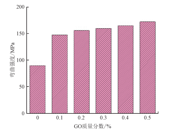
图 6 不同 GO 质量分数的 GO-CF 编织复合材料弯曲强度仿真结果 Fig. 6 Simulation results of bending strength for GO-CF woven composites with different GO mass fractions
