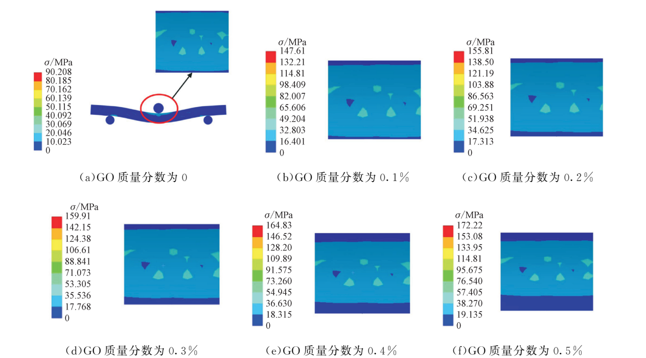
图 7 不同 GO 质量分数的 GO-CF 编织复合材料弯曲强度应力云图及局部放大图 Fig. 7 Stress cloud diagrams and local magnification images of bending strength for GO-CF woven composites with different GO mass fractions
